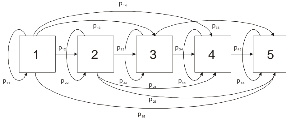
Figure 1. State transition diagram for five-state pipe example
