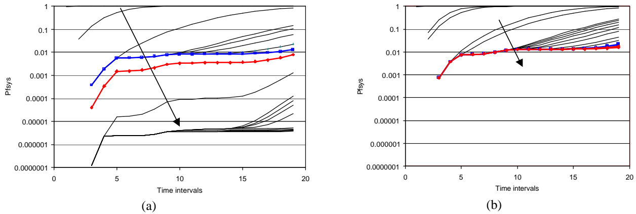
Figure 3. The cumulative probability of system failure for all of the OMS's shown in Table 3 (a) network 1 (b) network 2
